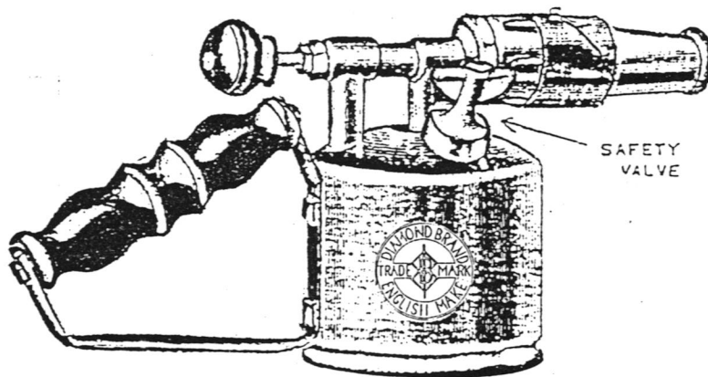
Petrol Blow Lamp Two-thirds pint.
