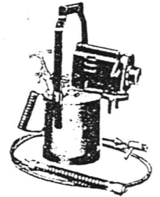
M79 "Monitor". Six-pint paraffin with pressure gauge, self-contained pump, safety device and flexible extension.
