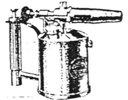
M46A "Monitor". One pint. Pump in handle and "Monitor" safety device. Horizontal burner. Self-cleaning needle.
