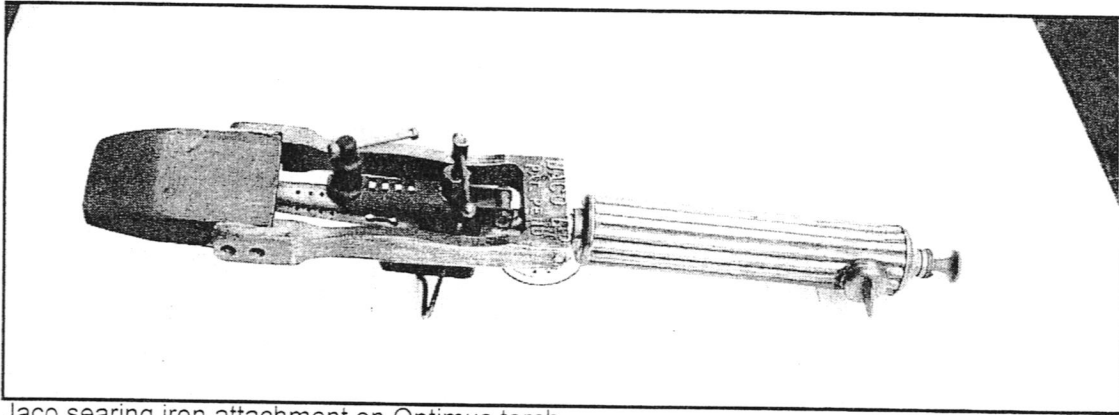
Jaco searing iron attachment on Optimus torch.
